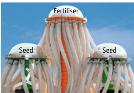
Distributor heads
